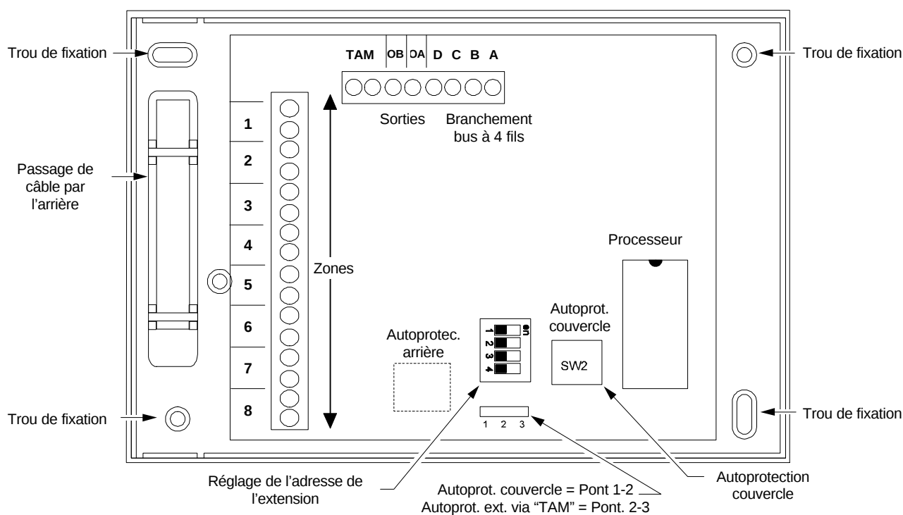
Figure 17. Extension CD9031S33
